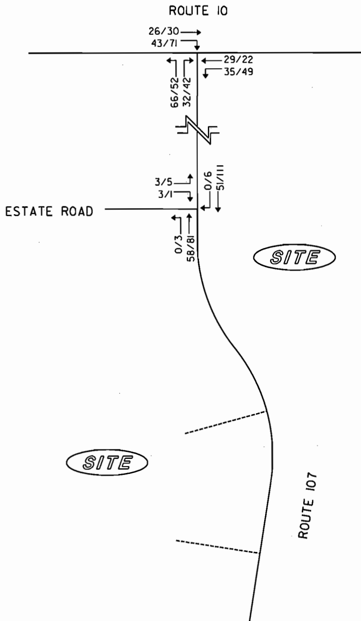
FIGURE 1 EXISTING FRIDAY PEAK HOUR TRAFFIC VOLUMES
